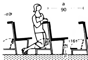
⑪ Seating in Roman Catholic church (with kneeler)
